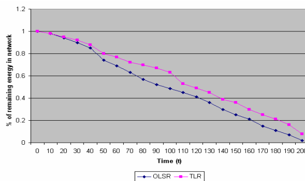
Figure 8. Percentage of remaining energy for networks running OLSR and TLR.
