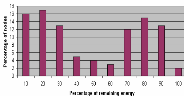
Figure 6. Energy distribution in nodes running OLSR.
